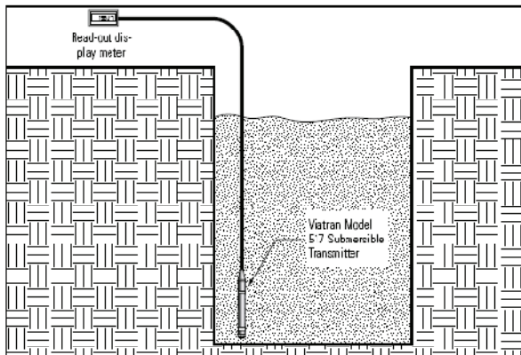
Diagram 2 – Open tank with a submersible transmitter.
