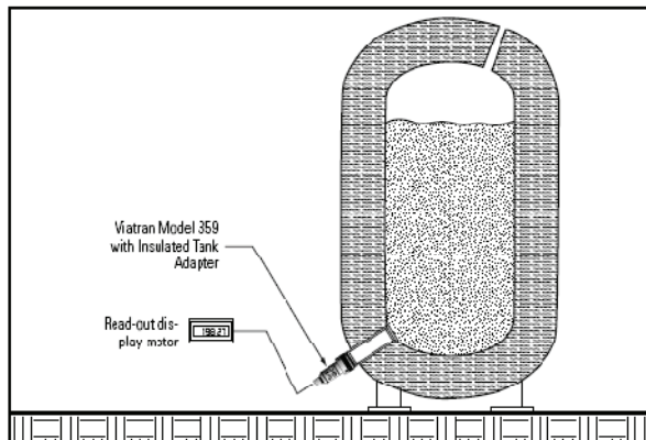
Diagram 3 – Insulated tank with adapter.
